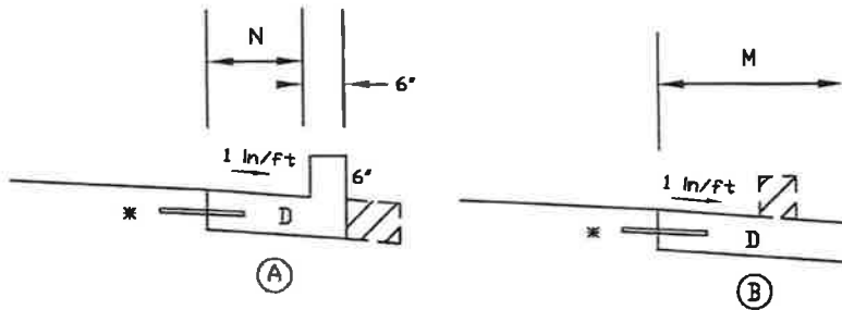
(B) EXTENDED GUTTER WITH NO CURB
