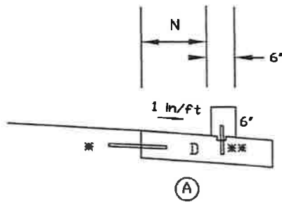
(A) EXTENDED GUTTER WITH 6 IN CURB
