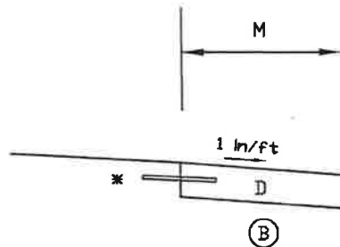
(B) EXTENDED GUTTER WITH NO CURB
